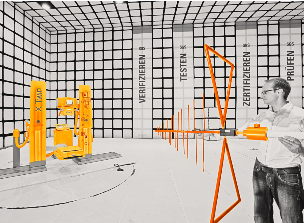
EMC Chamber Radiated Emission testing of an X-ray System.
